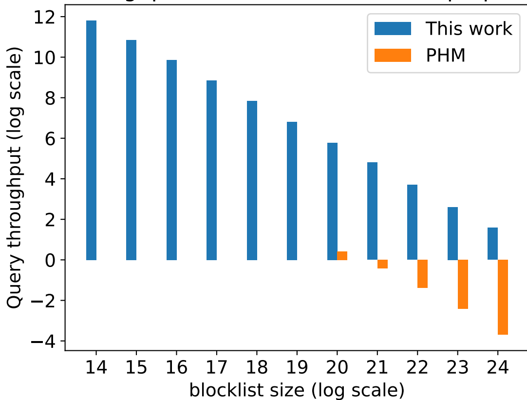
Server throughput vs. Blocklist size (after preprocessing)
